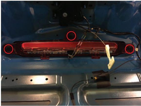
Step 3 Using a Phillips screw driver, remove the 3 plastic screw clips securing the factory brake light to the trunk. Then remove the brake light from the vehicle. Reinstall the Raxiom LED in reverse order.
