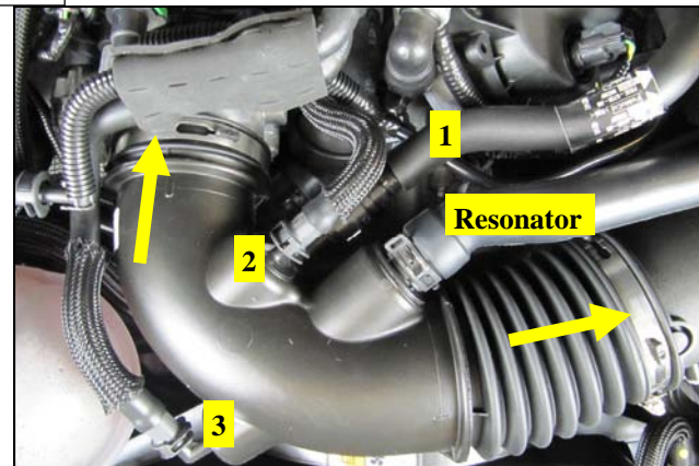
3. Disconnect the breather lines and resonator tube from the intake. Depending on your configuration, you may have two or three lines. Loosen the hose clamps and remove the factory intake tube.
