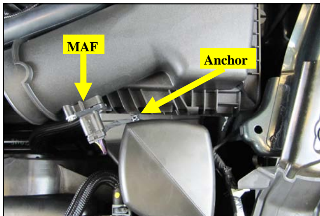
4. Gently pry the MAF harness anchor out of the airbox and disconnect the Mass Air Flow meter.
