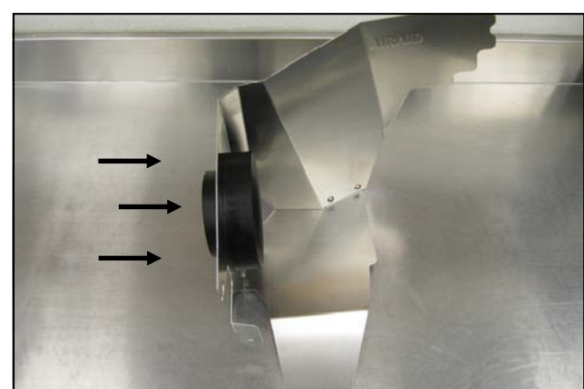
9. Install the Filter Adapter onto the Panel Assembly as shown, using the three 1/4-20 Button Head Screws and Flat Washers.
