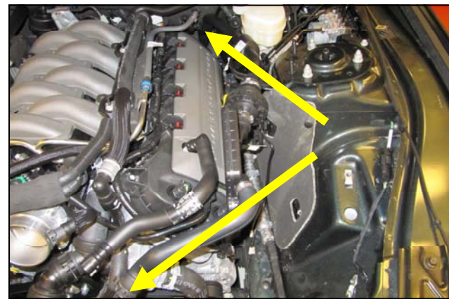
6. Remove the entire resonator assembly from the vehicle. It is held in place with two plastic retainers and a single 6mm nut on the firewall.
