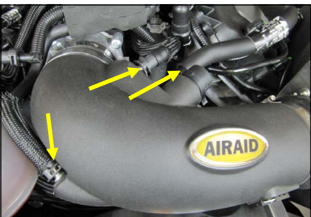
19. Insert the Intake Tube into the Hump Hose and Reducer then tighten all 4 Intake Clamps. Reconnect the factory breather lines. Apply the Airaid Bubble Decal onto the Intake Tube as shown.
