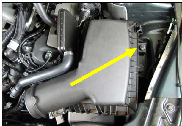
5. Remove the 6mm airbox mounting bolt in the inner fender and lift the entire airbox assembly out of the vehicle. Set the bolt aside for now. It will be reused.
