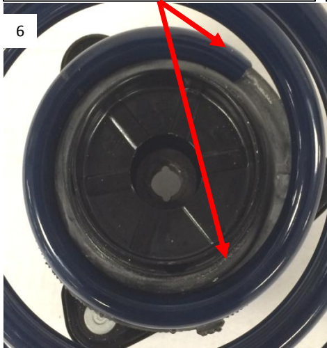
Correct , notice how the coil wraps 3/4 of the way around the upper spring seat.
