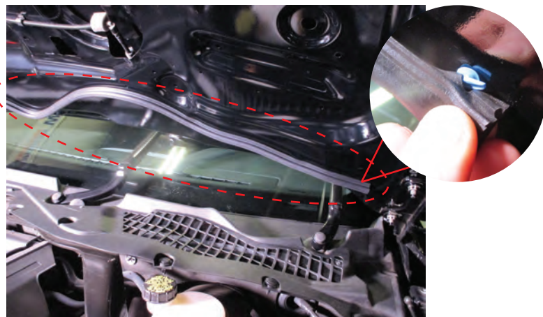
Step 2\\ Remove the cowl weather stripping.
