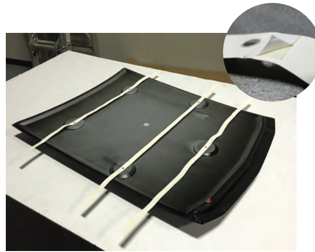
Step 3\\ Remove the adhesive tab on the supplied drilling templates, and stick them on the hood scoop.
