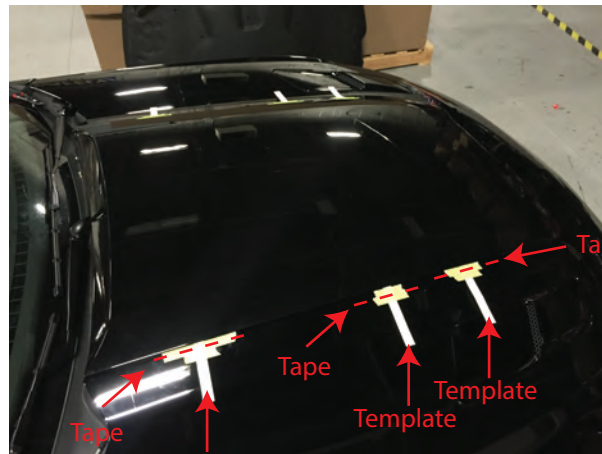
Step 5\\ Tape the template to the hood as close to the edge of the scoop as possible. Repeat this process for all template mounting locations. (3) On both sides.
