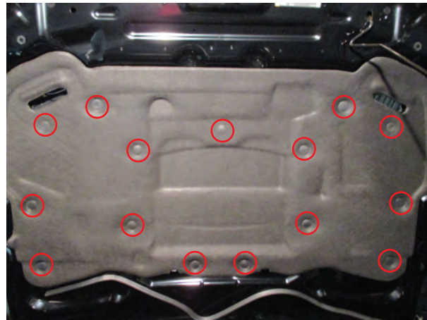
Step 1\\ Remove the 15 plastic retainers holding on the hood liner.
