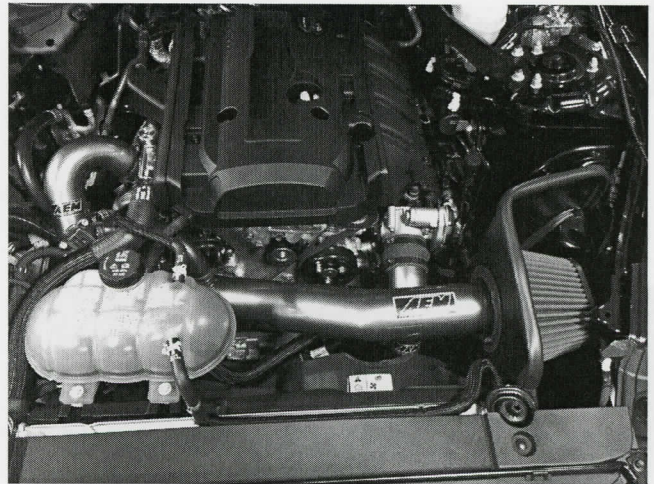
Finished installation of AEM Charge Pipe System (shown with AEM Intake System 21-740C.)
