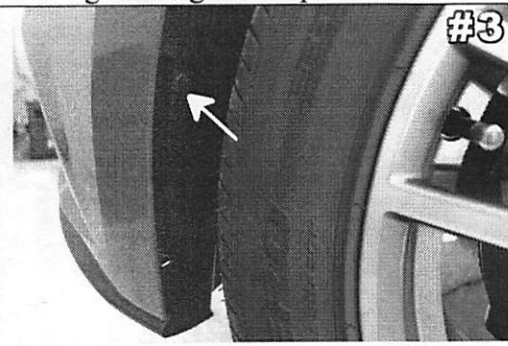
Remove push pin shown on right and left side front wheel well.
