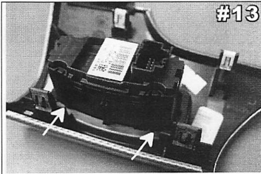
4 clips hold switch in. 2 clips are shown above.
