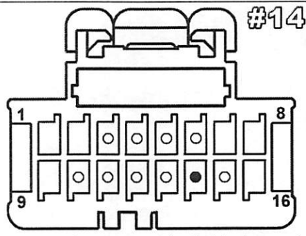
Connect wire tap to pin # 14 shown by solid black dot above.
