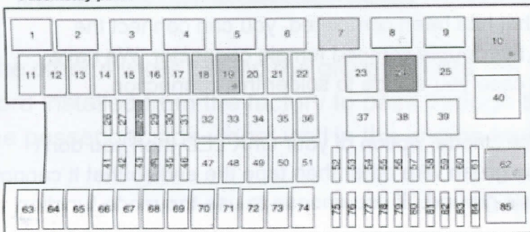
Fuse/Relay panel
